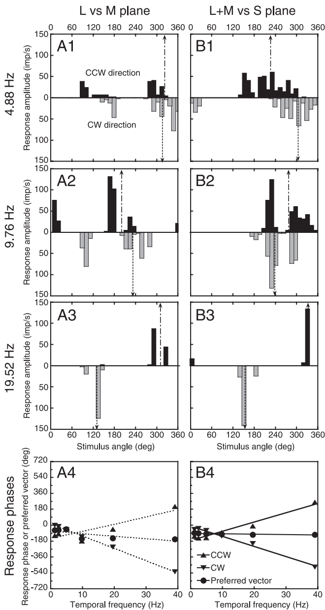
FIG. 9. Responses of an OFF-center MC ganglion cell. Format is similar to Fig. 4. For modulation in the L- vs. M-cone plane, the cell's preferred vector was in the opponent quadrant at low frequency but moved to the achromatic quadrant at higher frequencies. Linear fit for preferred vectors in this plane (dashed line) is drawn only to show the nonzero slope.
